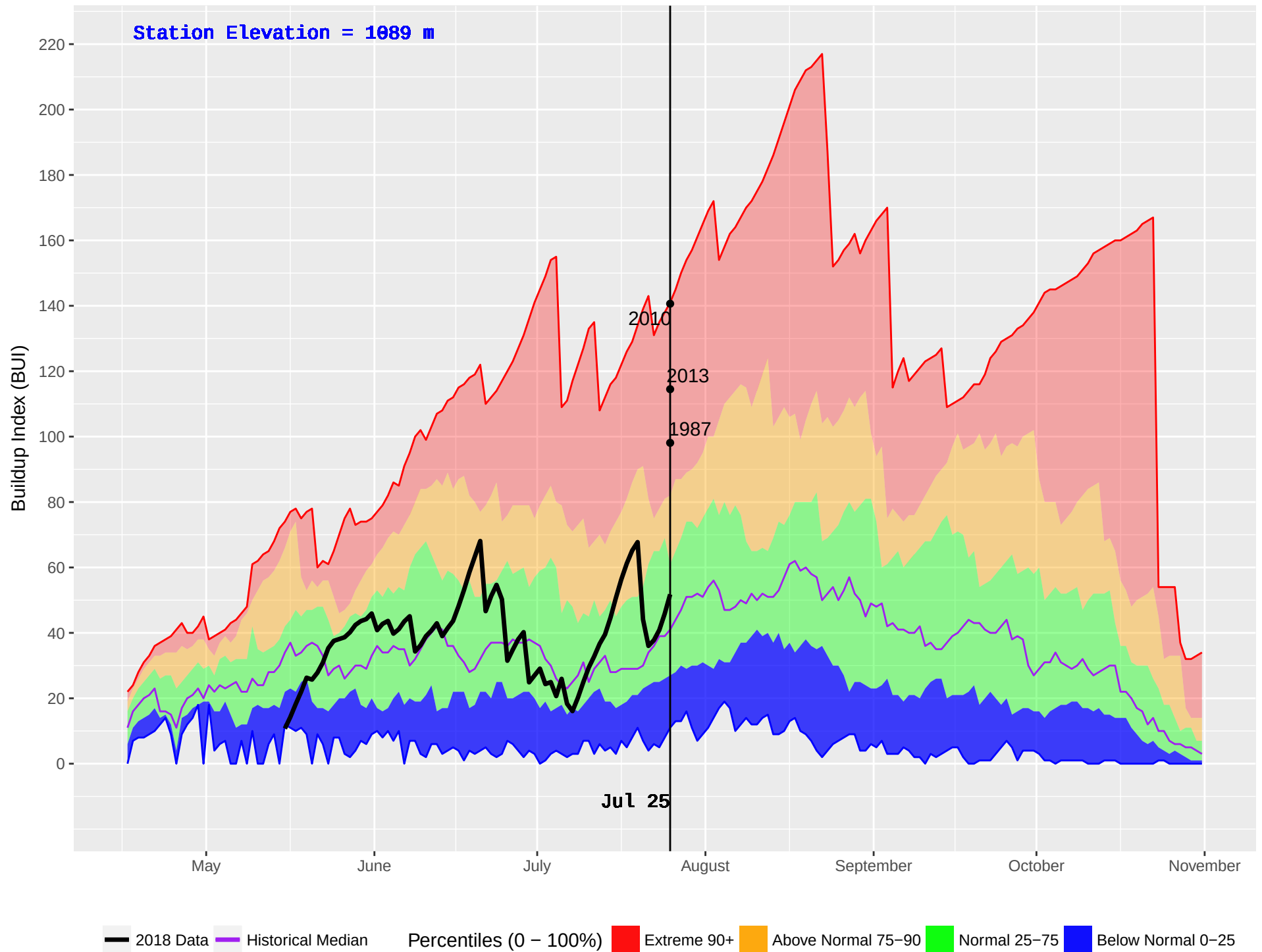
EAST OOTSA (170) : Historical (1986–2016) and Current (2018) Noon Buildup Index (BUI)
