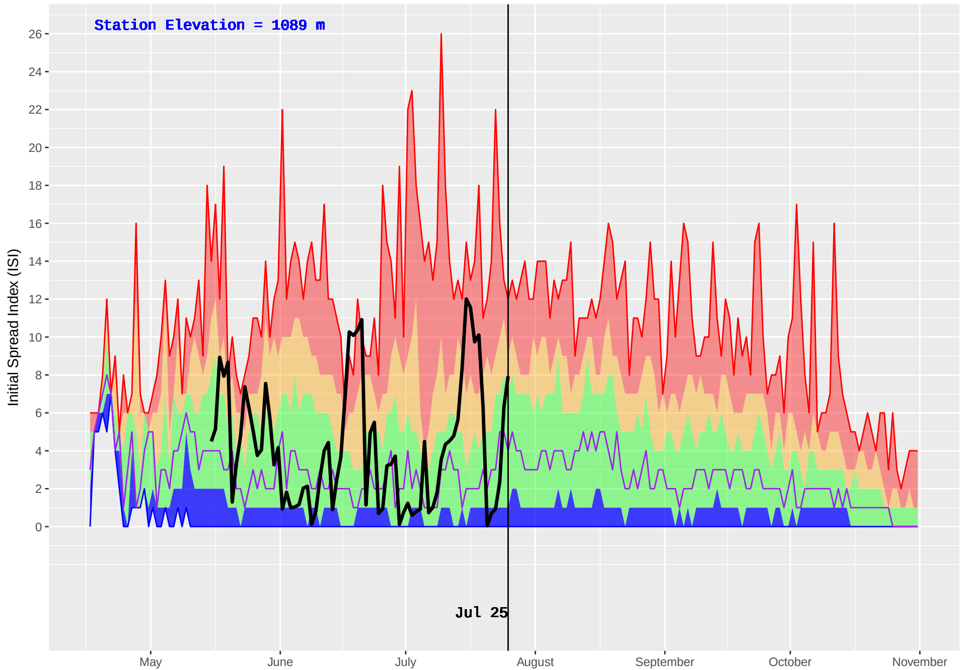
EAST OOTSA (170) : Historical (1986–2016) and Current (2018) Noon Initial Spread Index (ISI)
